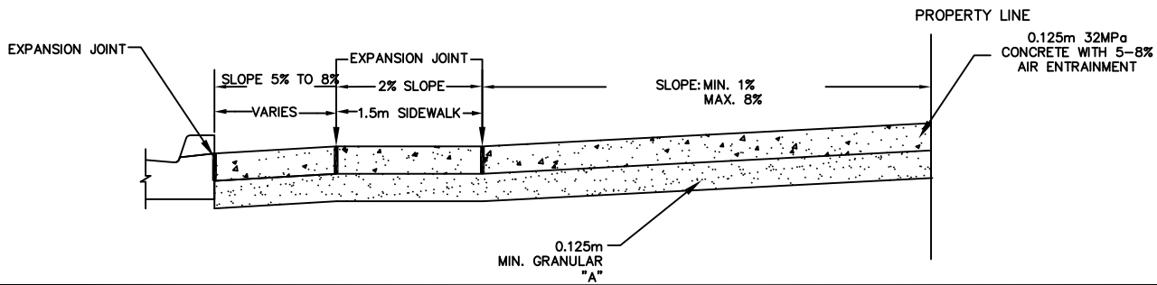
SECTION B-B CONCRETE
