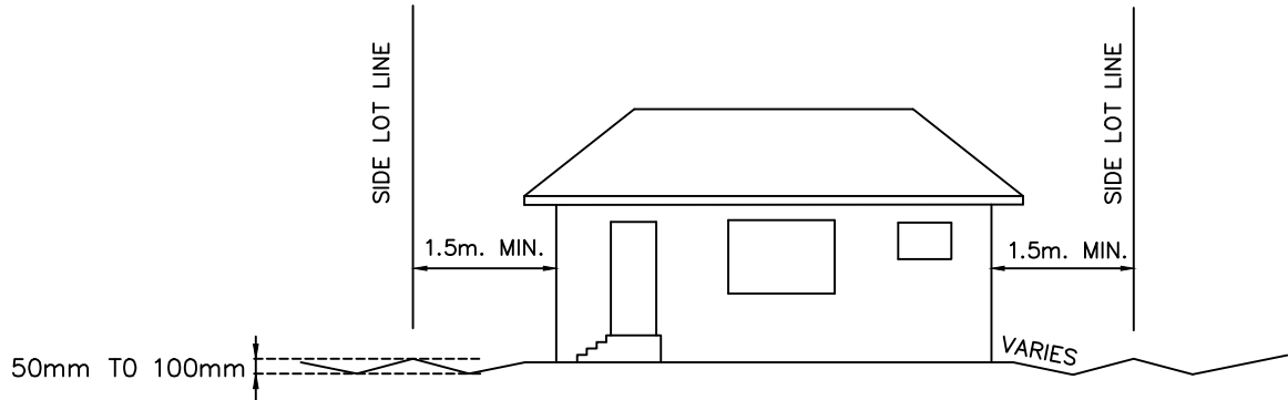
SECTION THROUGH SIDE YARDS
