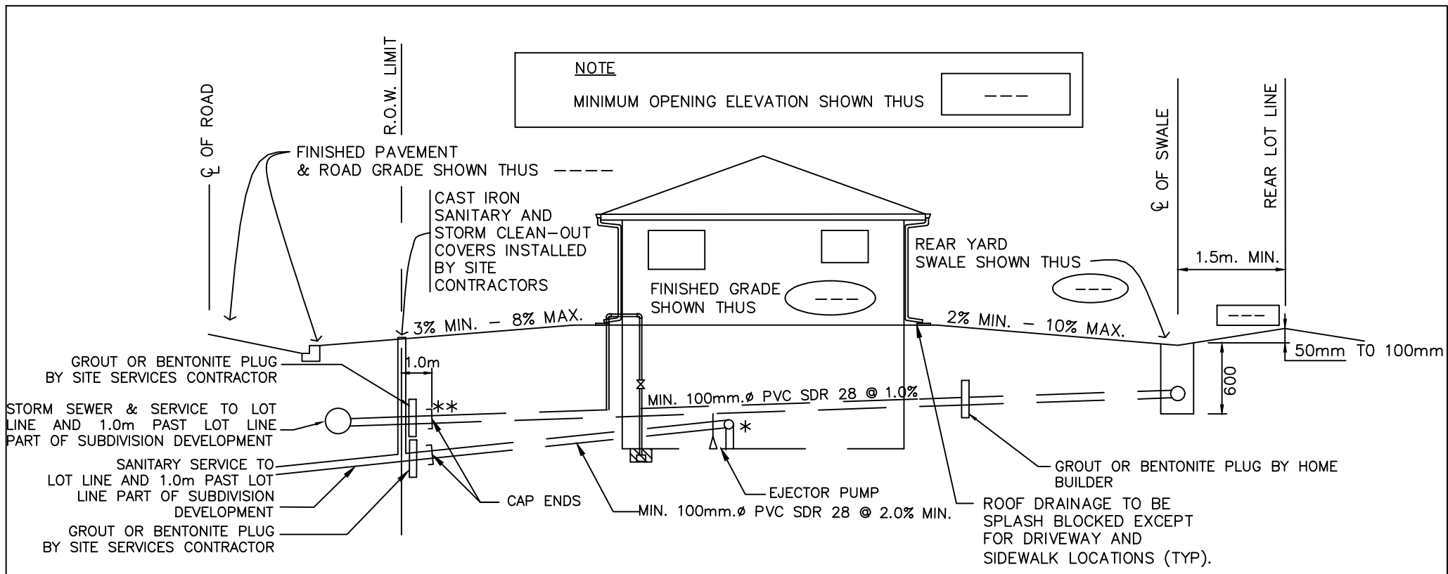
SECTION THROUGH FRONT & REAR YARDS
